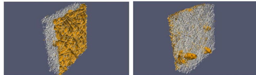
Oil interface in filter medium - inlet side
