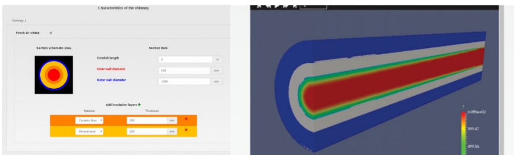
HPC-based simulation
